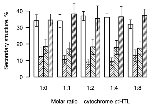
FIGURE 7: Secondary structure composition of N-Hcy-cytochrome c modified with increasing molar excess of HTL. The mean percentages of each structural element, \alpha -helix (empty bars), \beta -sheet (//), turns (\\), and unordered (dotted bars) in unmodified and HTL-modified cytochrome c , calculated from corresponding CD spectra, are shown.
